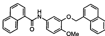
Compound # 47
